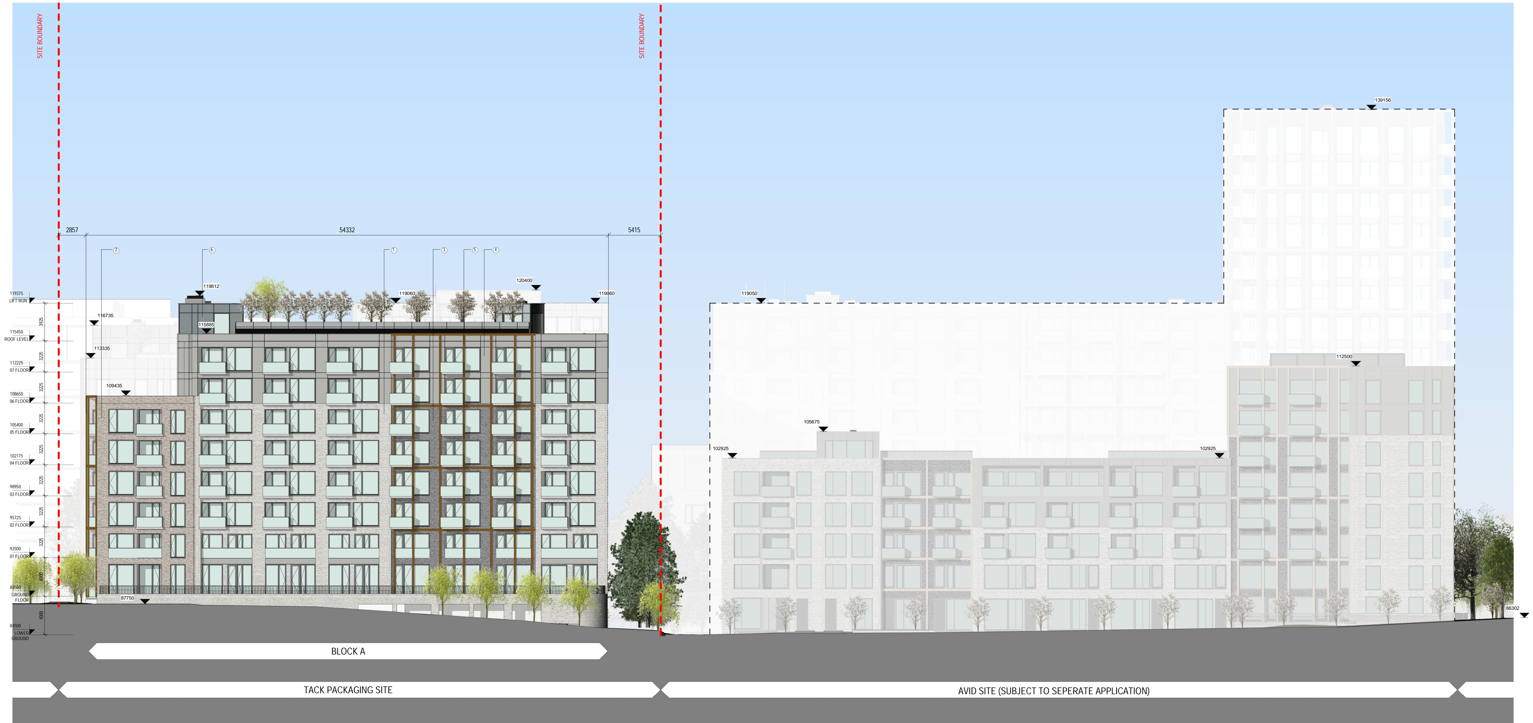
1 PROPOSED SOUTH WEST ELEVATION - TACK SITE 1 : 200
